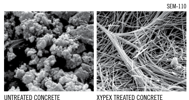
UNTREATED CONCRETE XYPEX TREATED CONCRETE
